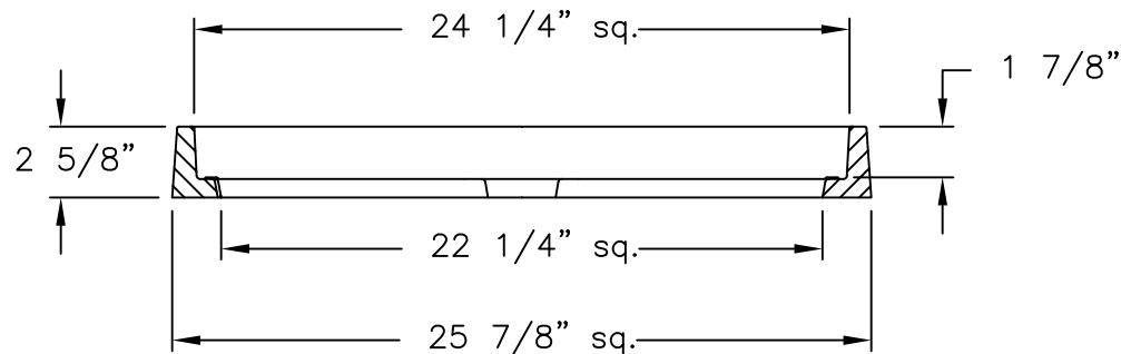
FRAME SECTION
